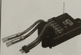
BSC/Receiver(The Waterproof Gcuc Has Been Poured)
